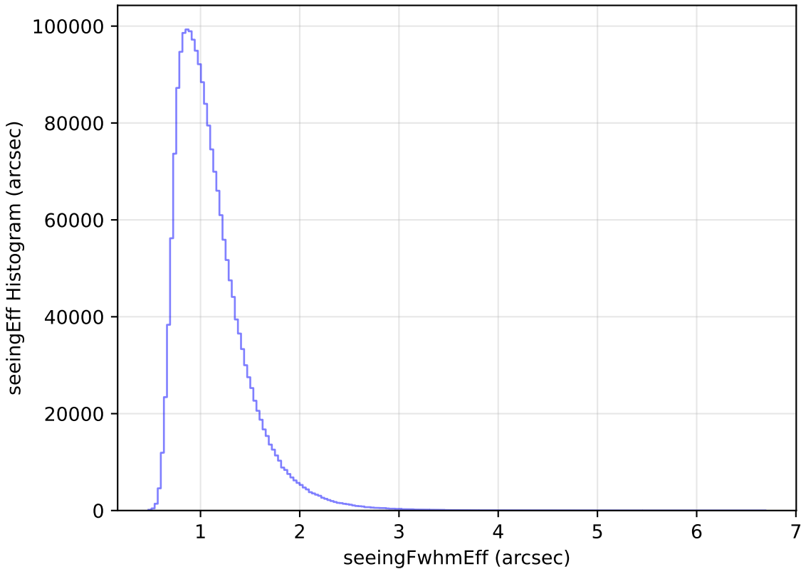
too_ignore_100_4v3.4_10yrs WFD all bands: seeingEff Histogram
