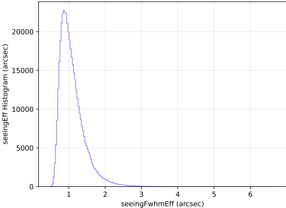
too_ignore_100_4v3.4_10yrs All sky z band: seeingEff Histogram
