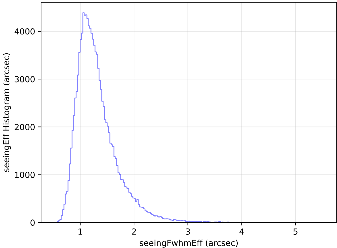
too_ignore_100_4v3.4_10yrs All sky u band: seeingEff Histogram
