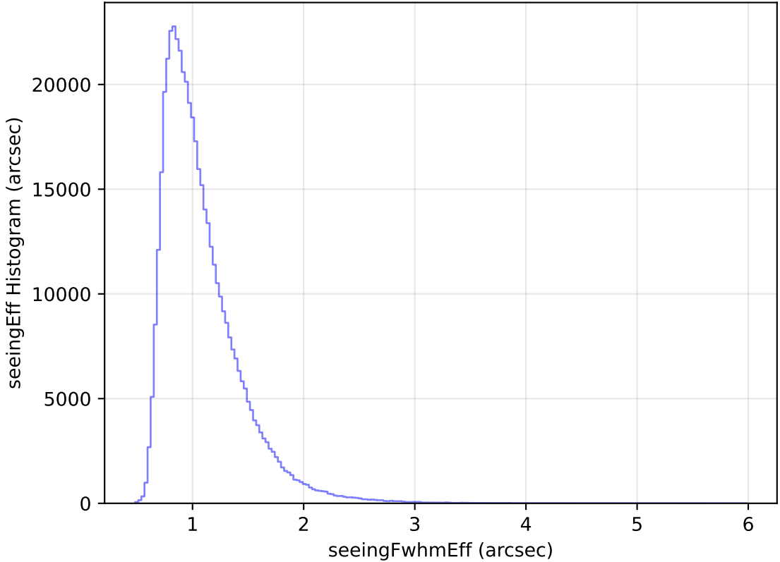
too_ignore_100_4v3.4_10yrs All sky i band: seeingEff Histogram
