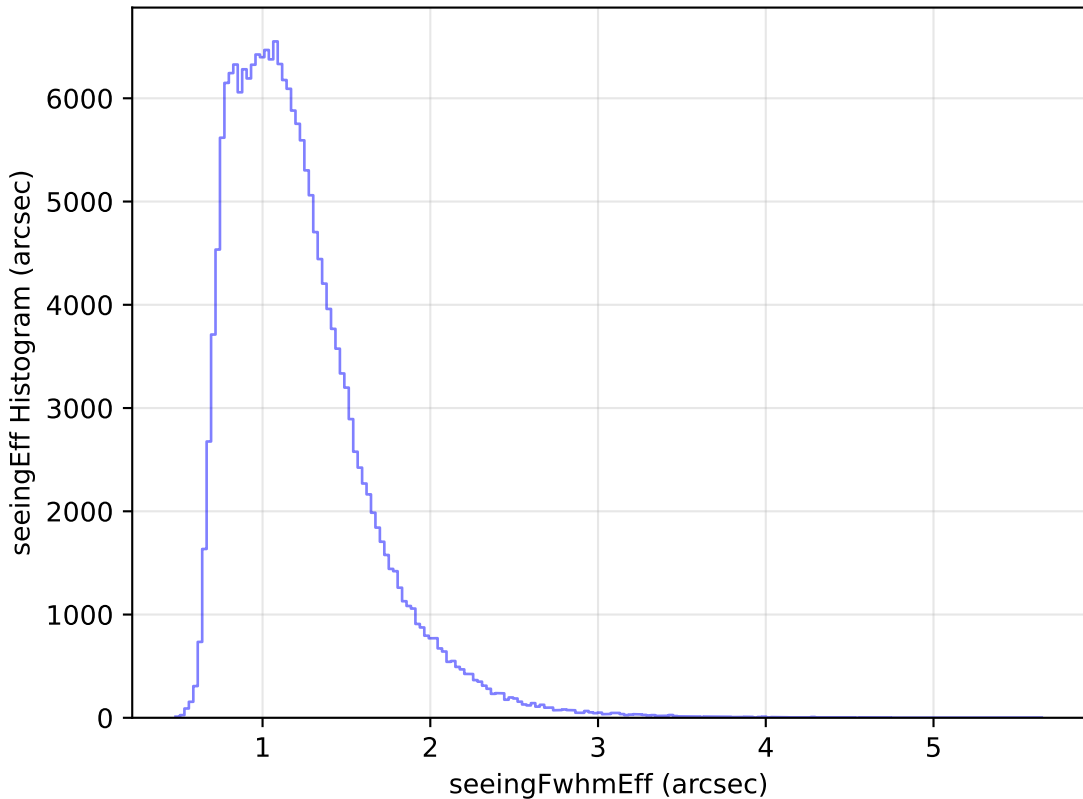
too_ignore_100_4v3.4_10yrs All sky g band: seeingEff Histogram
