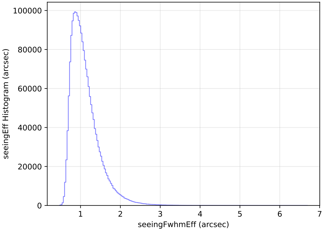
too_ignore_100_4v3.4_10yrs All sky all bands: seeingEff Histogram
