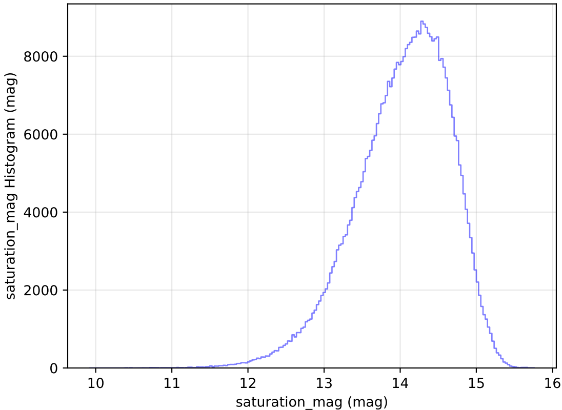
too_ignore_100_4v3.4_10yrs WFD z band: saturation_mag Histogram
