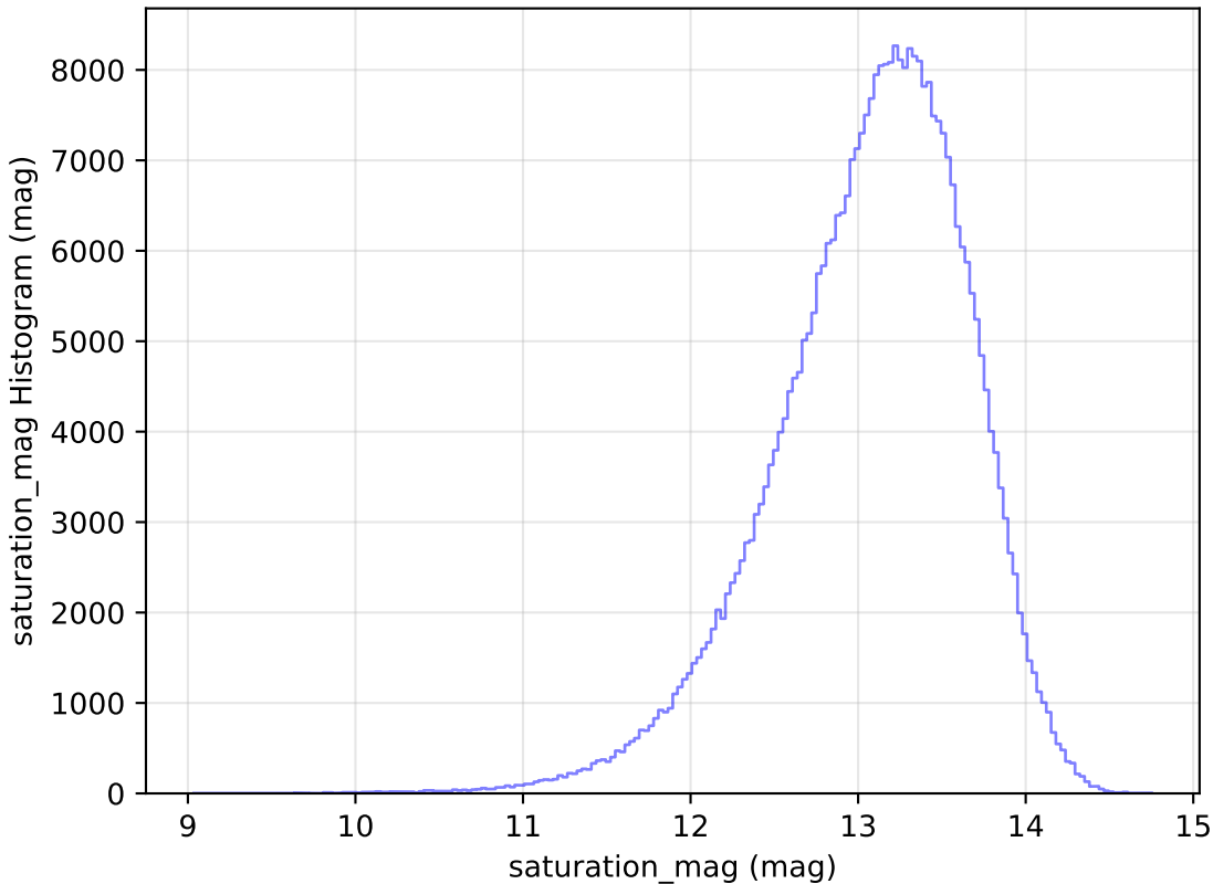
too_ignore_100_4v3.4_10yrs WFD y band: saturation_mag Histogram
