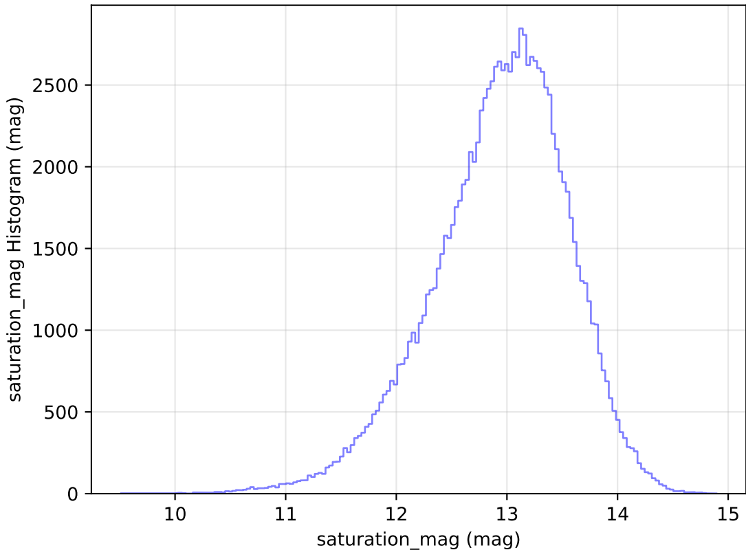
too_ignore_100_4v3.4_10yrs WFD u band: saturation_mag Histogram
