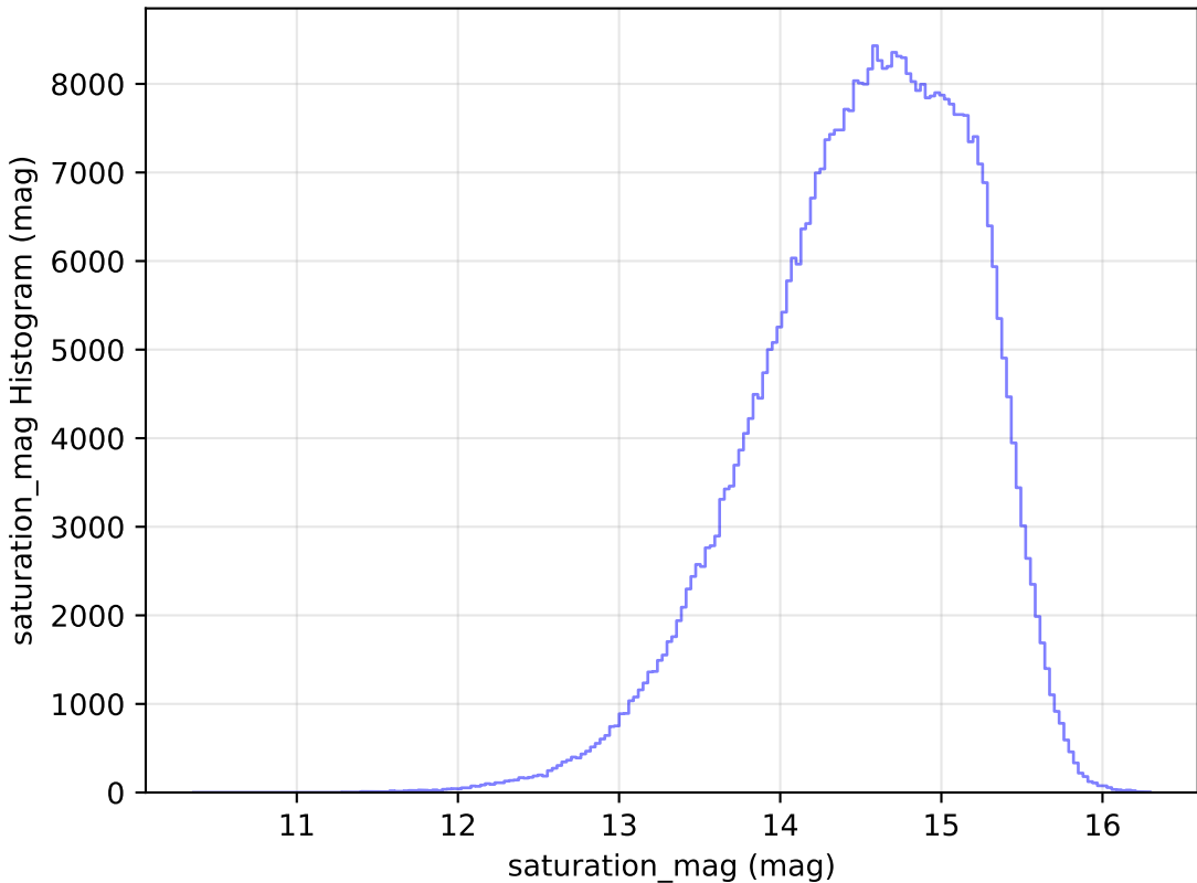
too_ignore_100_4v3.4_10yrs WFD r band: saturation_mag Histogram
