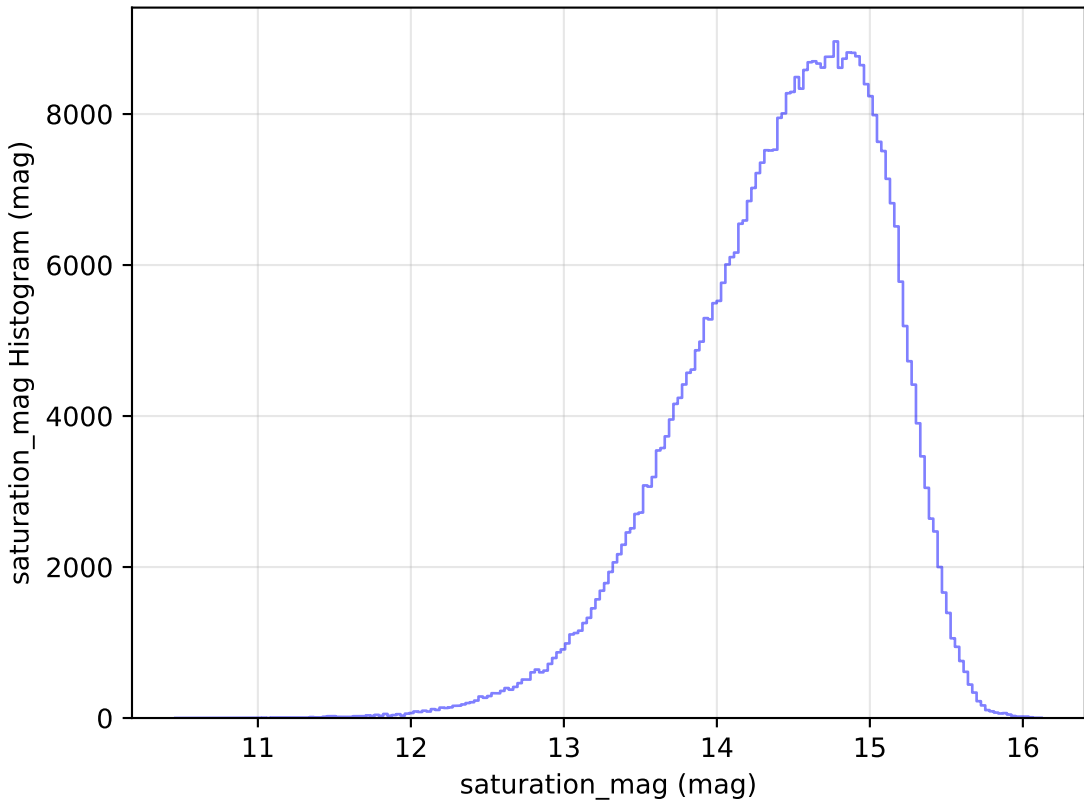
too_ignore_100_4v3.4_10yrs WFD i band: saturation_mag Histogram
