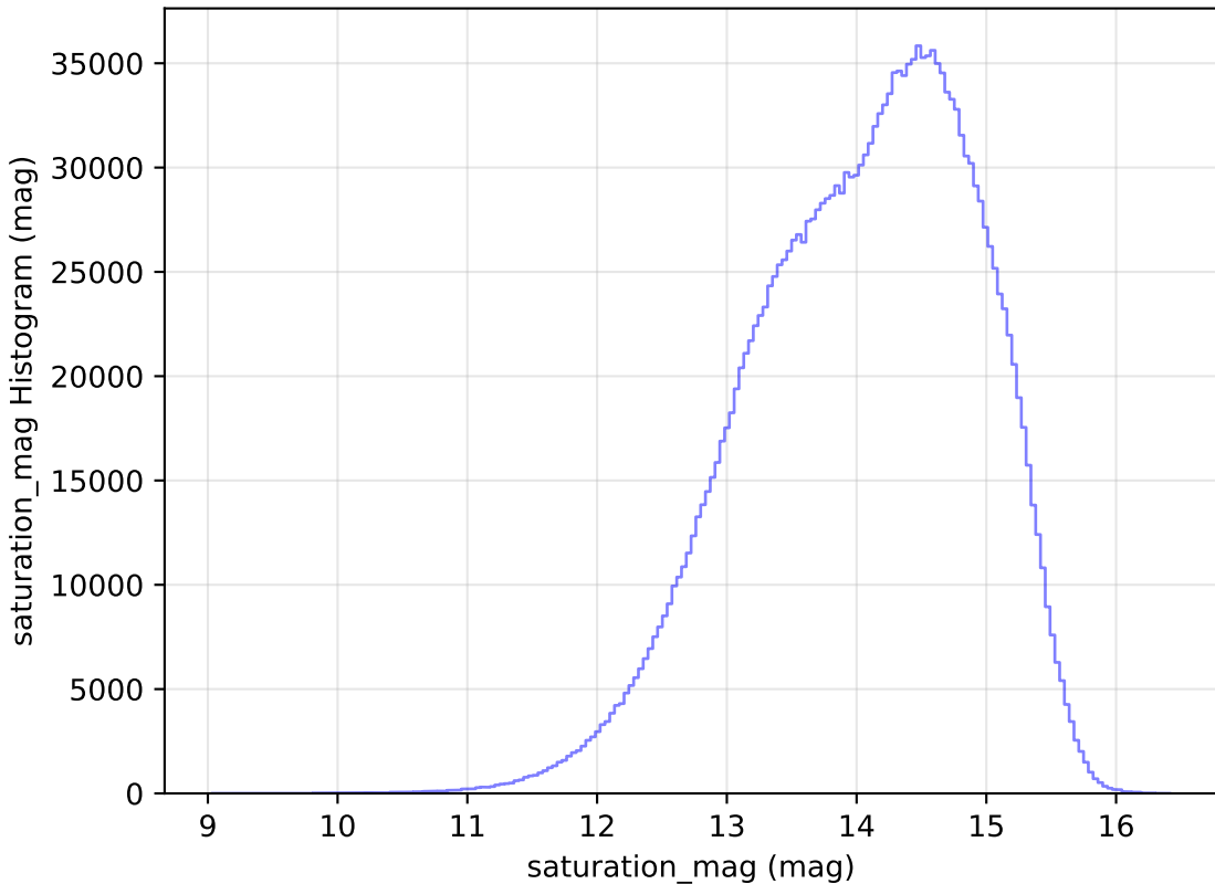
too_ignore_100_4v3.4_10yrs WFD all bands: saturation_mag Histogram
