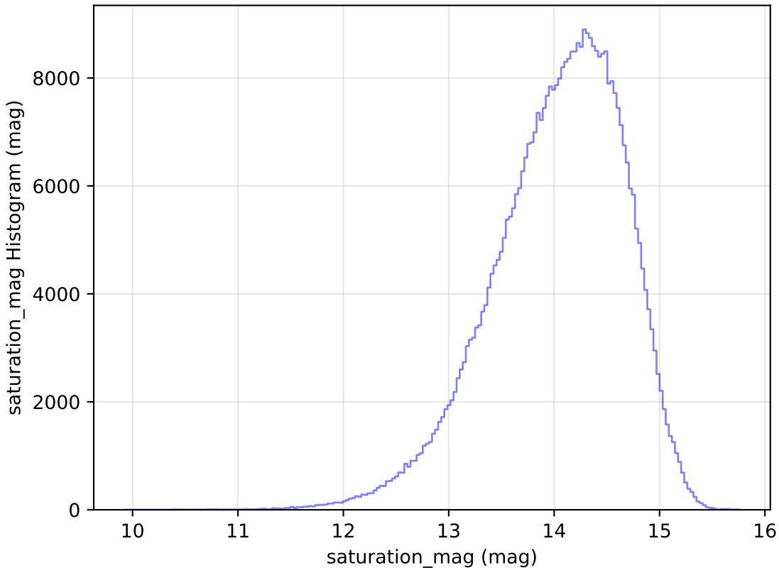
too_ignore_100_4v3.4_10yrs All sky z band: saturation_mag Histogram
