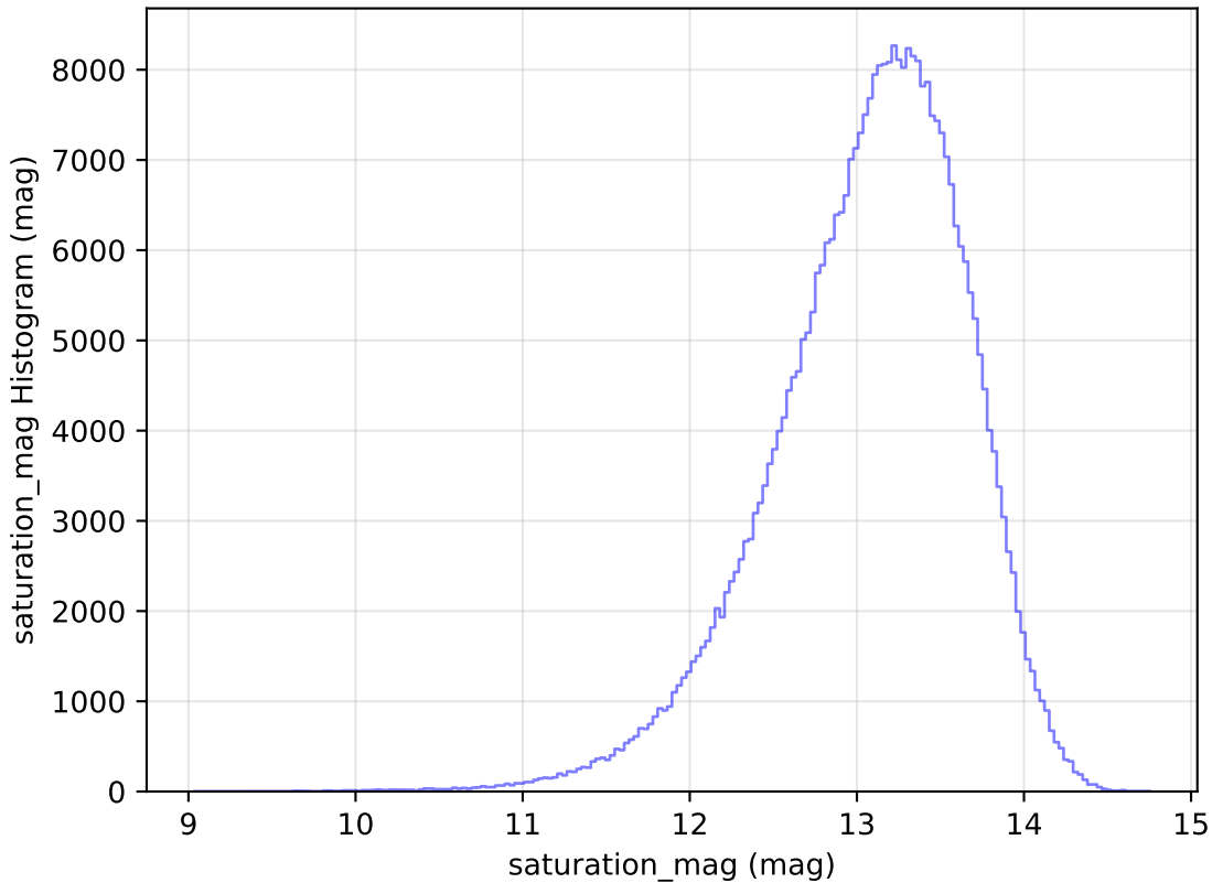
too_ignore_100_4v3.4_10yrs All sky y band: saturation_mag Histogram
