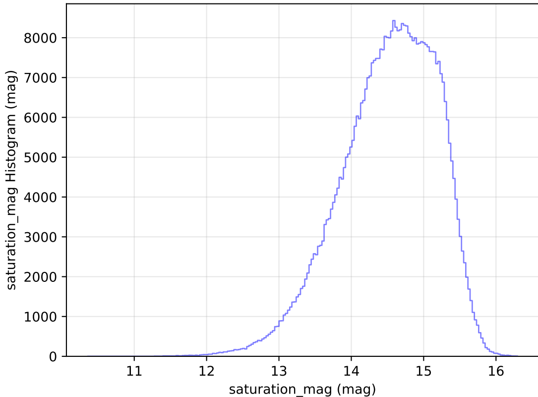
too_ignore_100_4v3.4_10yrs All sky r band: saturation_mag Histogram
