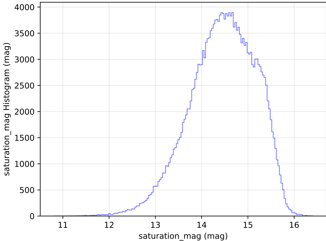
too_ignore_100_4v3.4_10yrs All sky g band: saturation_mag Histogram
