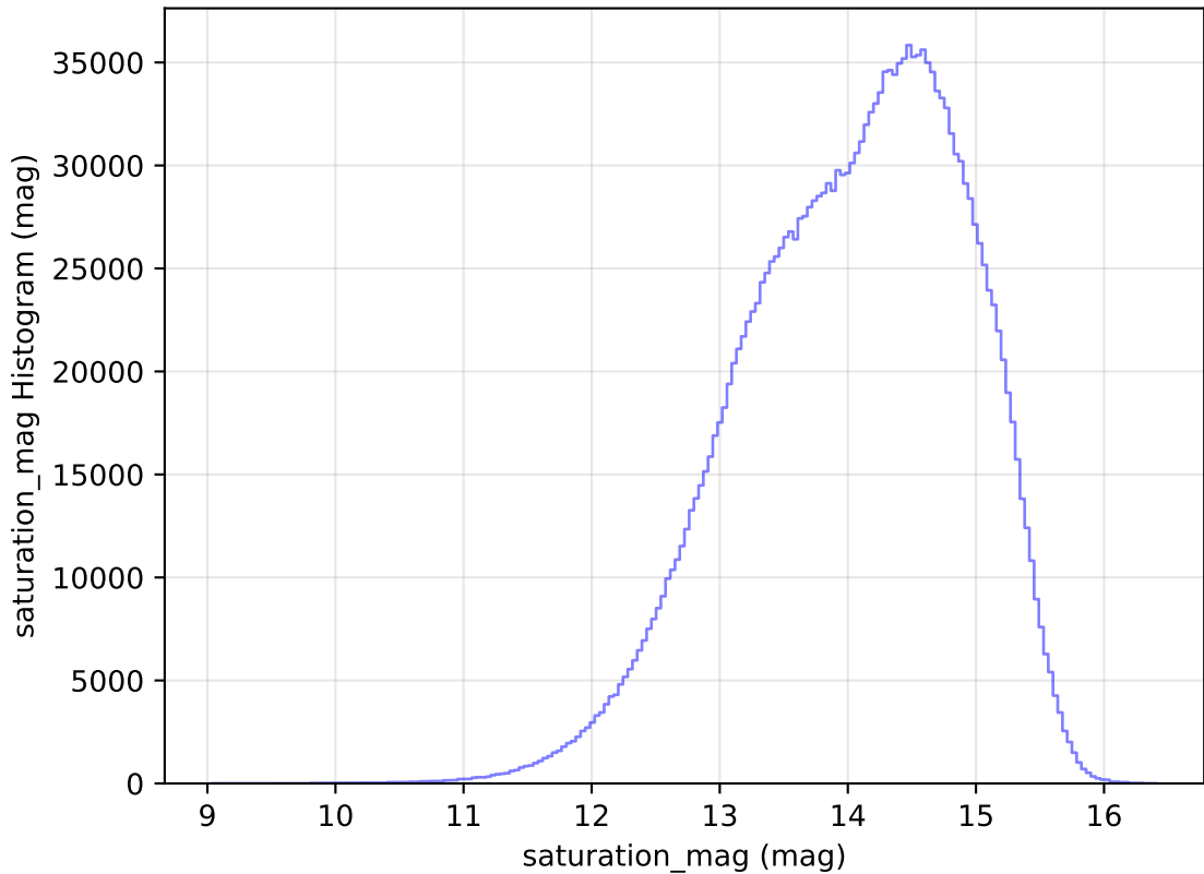
too_ignore_100_4v3.4_10yrs All sky all bands: saturation_mag Histogram
