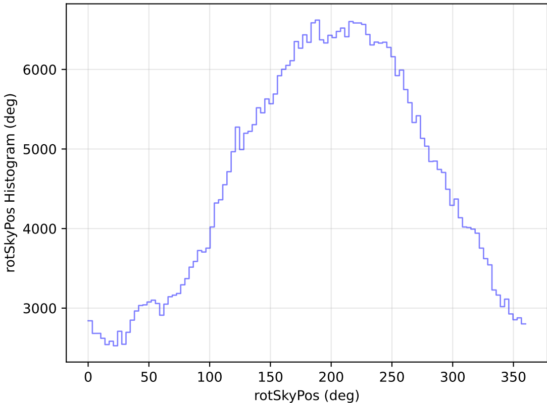
too_ignore_100_4v3.4_10yrs WFD r band: rotSkyPos Histogram
