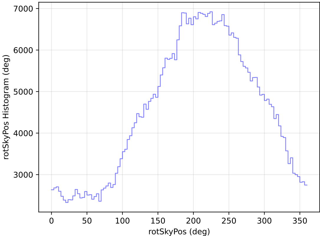
too_ignore_100_4v3.4_10yrs WFD i band: rotSkyPos Histogram
