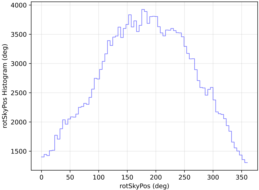
too_ignore_100_4v3.4_10yrs WFD g band: rotSkyPos Histogram
