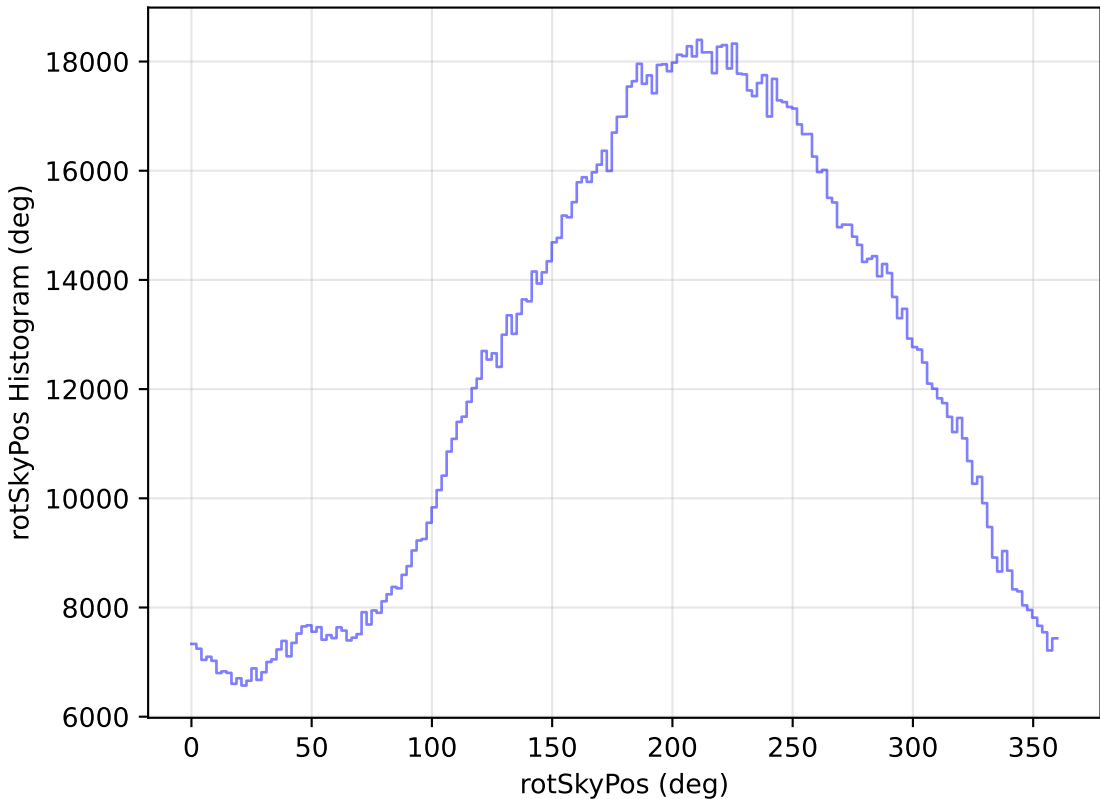
too_ignore_100_4v3.4_10yrs WFD all bands: rotSkyPos Histogram
