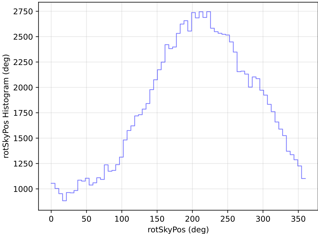
too_ignore_100_4v3.4_10yrs All sky u band: rotSkyPos Histogram
