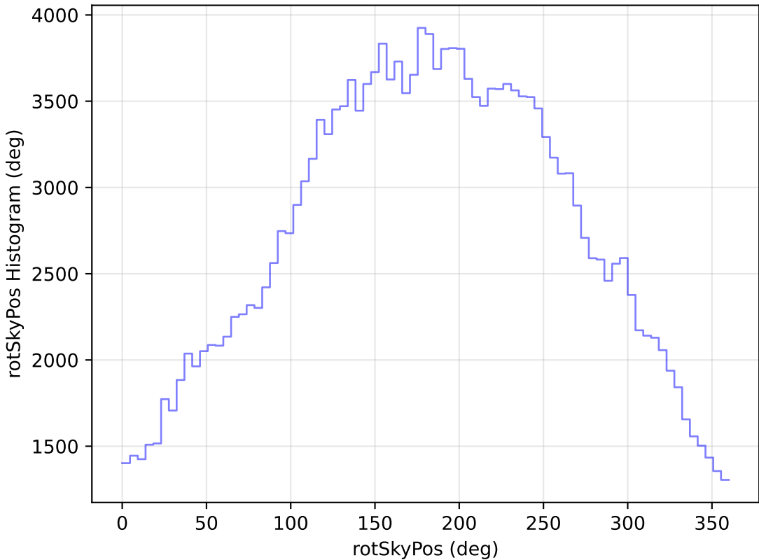
too_ignore_100_4v3.4_10yrs All sky g band: rotSkyPos Histogram
