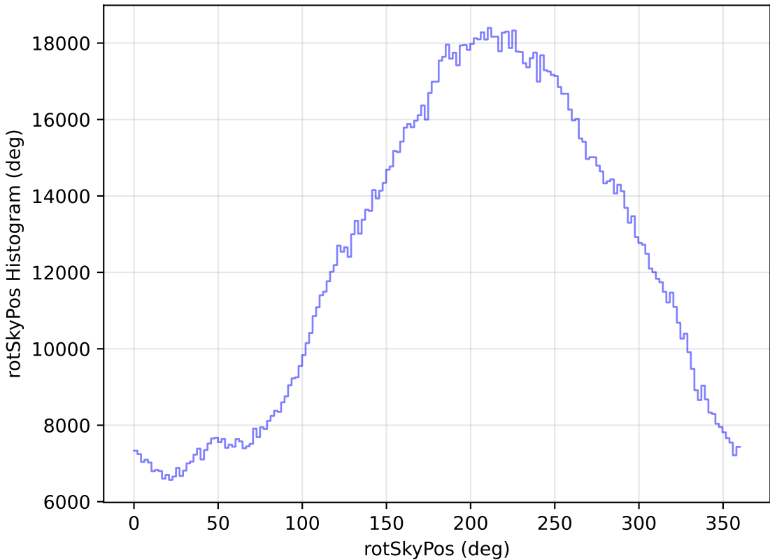
too_ignore_100_4v3.4_10yrs All sky all bands: rotSkyPos Histogram
