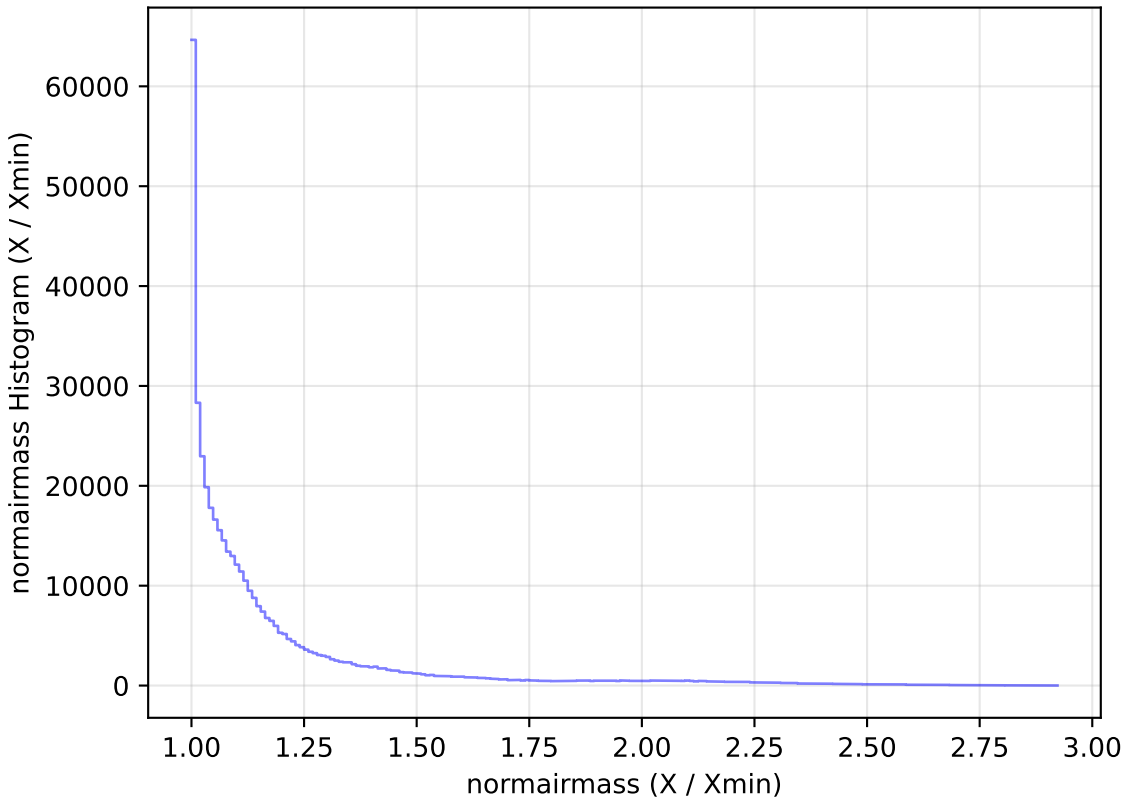
too_ignore_100_4v3.4_10yrs WFD z band: normairmass Histogram
