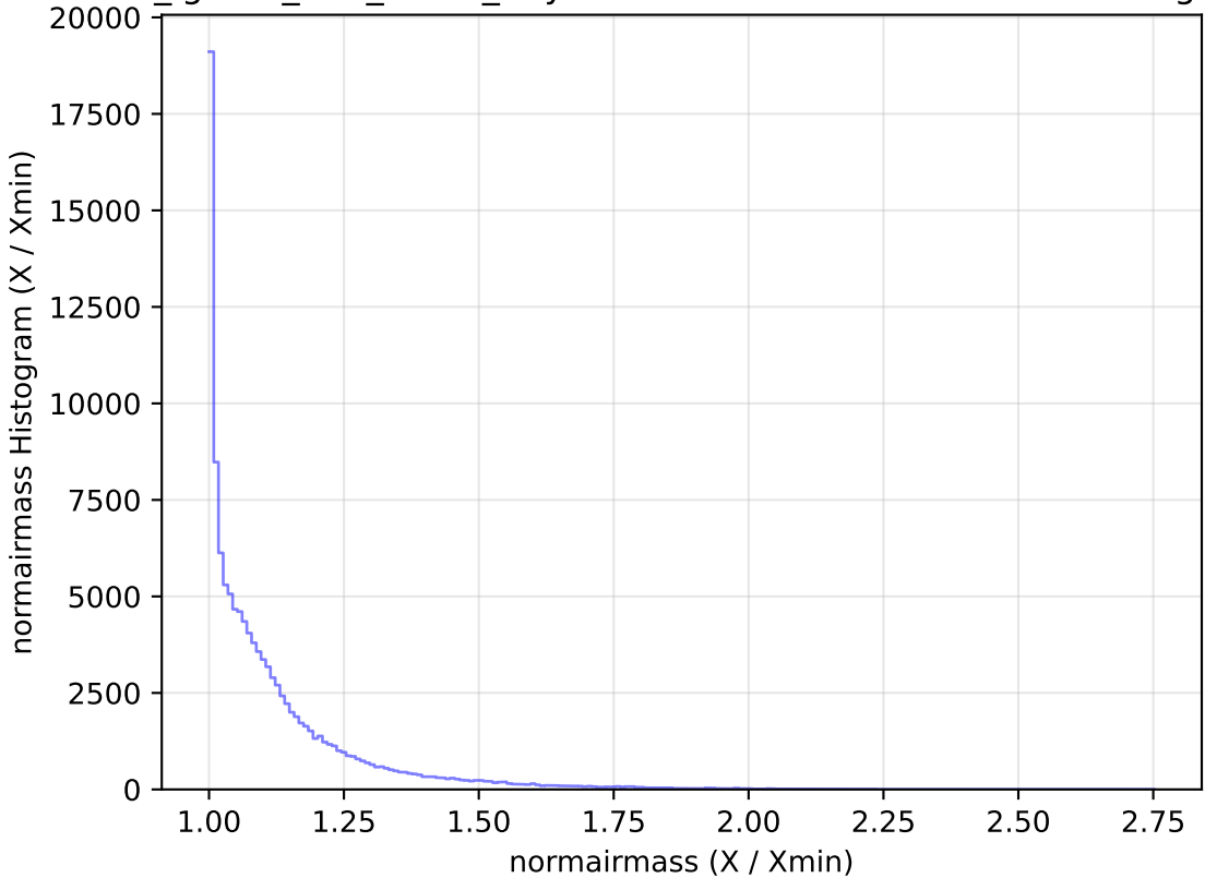
too_ignore_100_4v3.4_10yrs WFD u band: normairmass Histogram
