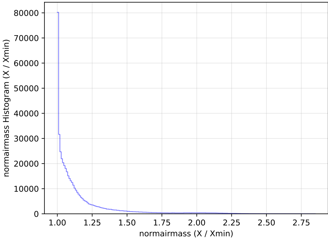
too_ignore_100_4v3.4_10yrs WFD r band: normairmass Histogram
