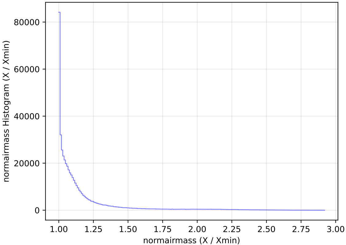
too_ignore_100_4v3.4_10yrs WFD i band: normairmass Histogram
