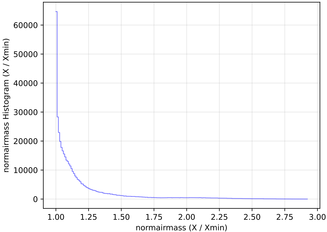
too_ignore_100_4v3.4_10yrs All sky z band: normairmass Histogram
