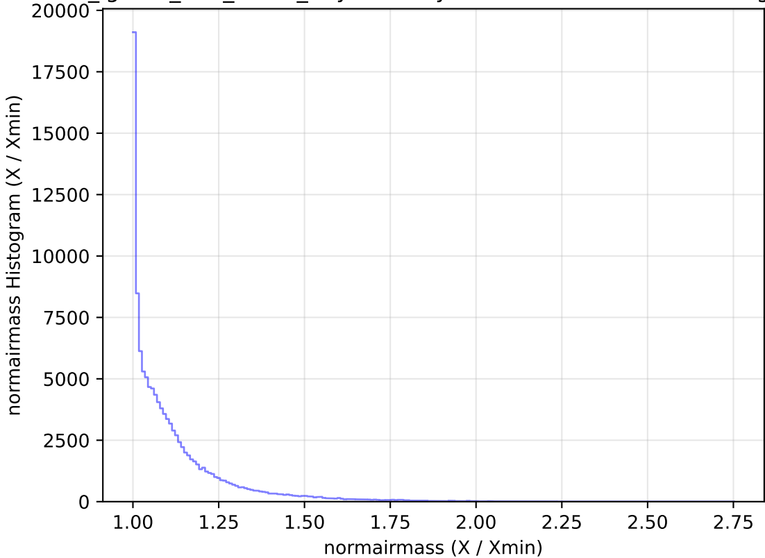
too_ignore_100_4v3.4_10yrs All sky u band: normairmass Histogram
