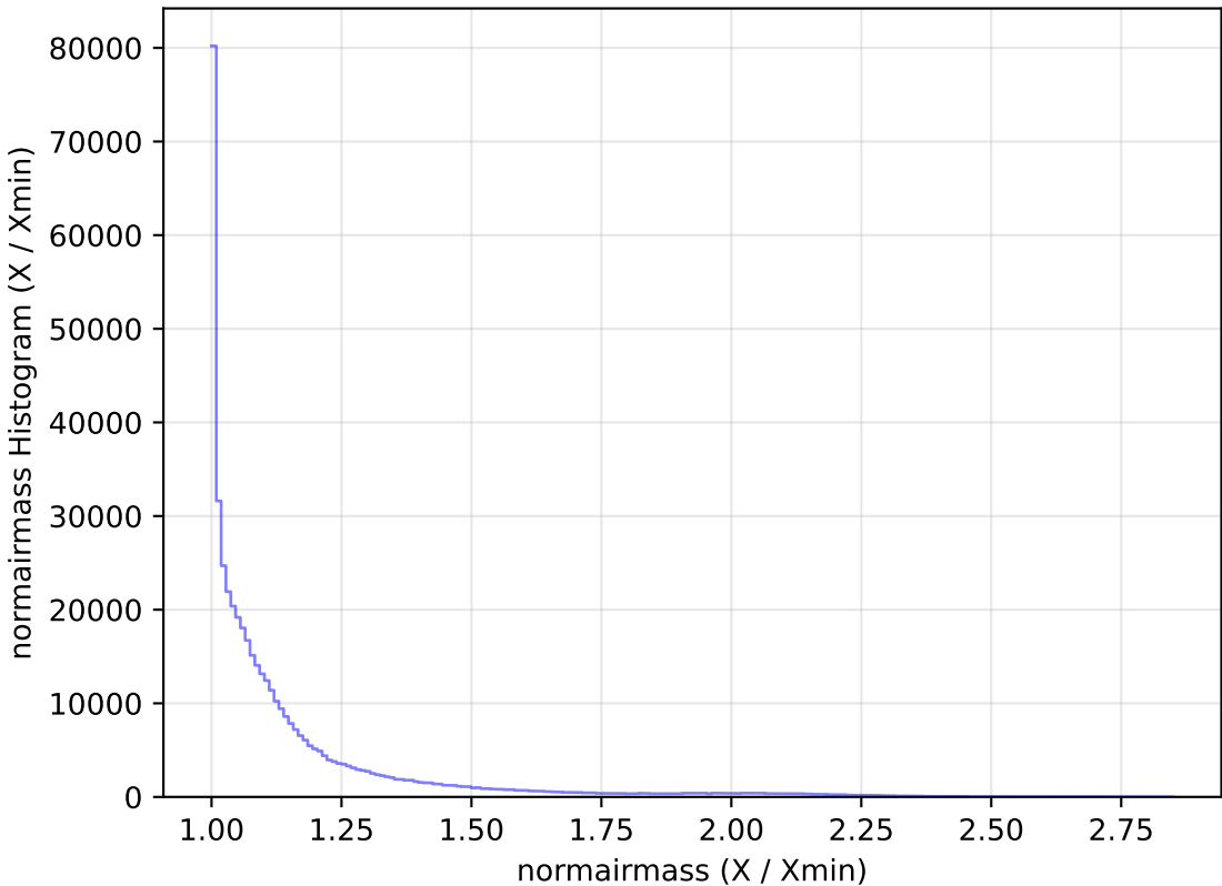
too_ignore_100_4v3.4_10yrs All sky r band: normairmass Histogram
