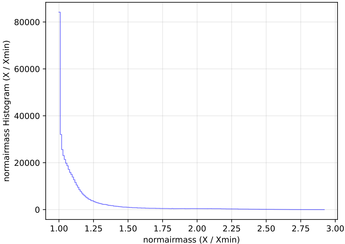
too_ignore_100_4v3.4_10yrs All sky i band: normairmass Histogram
