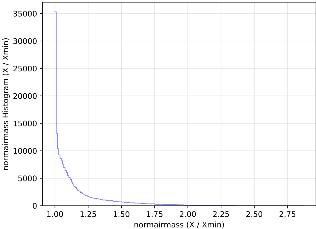
too_ignore_100_4v3.4_10yrs All sky g band: normairmass Histogram
