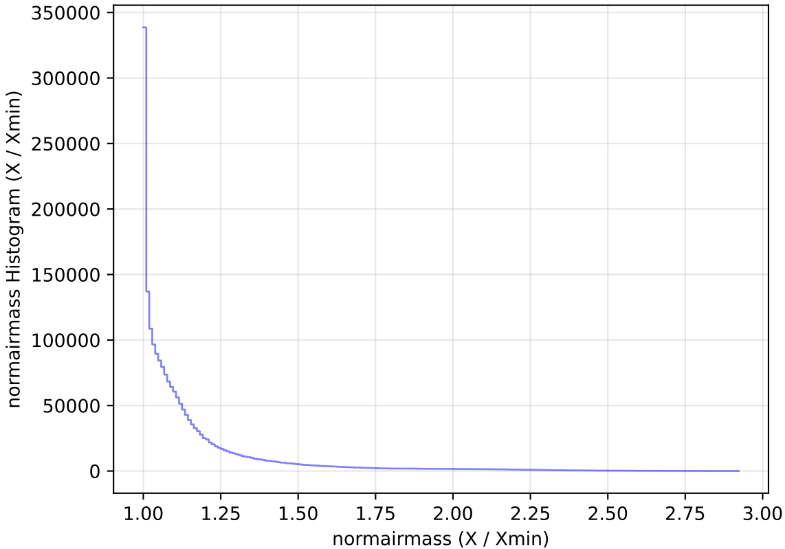
too_ignore_100_4v3.4_10yrs All sky all bands: normairmass Histogram
