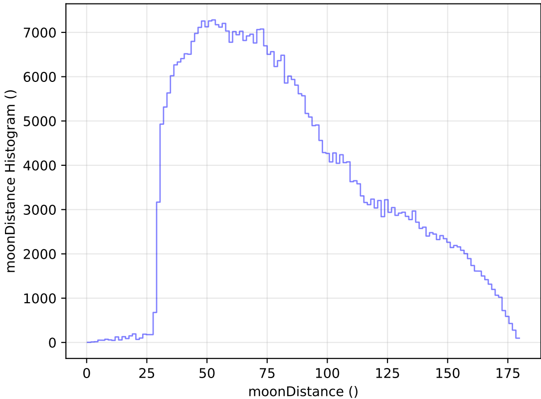
too_ignore_100_4v3.4_10yrs WFD z band: moonDistance Histogram
