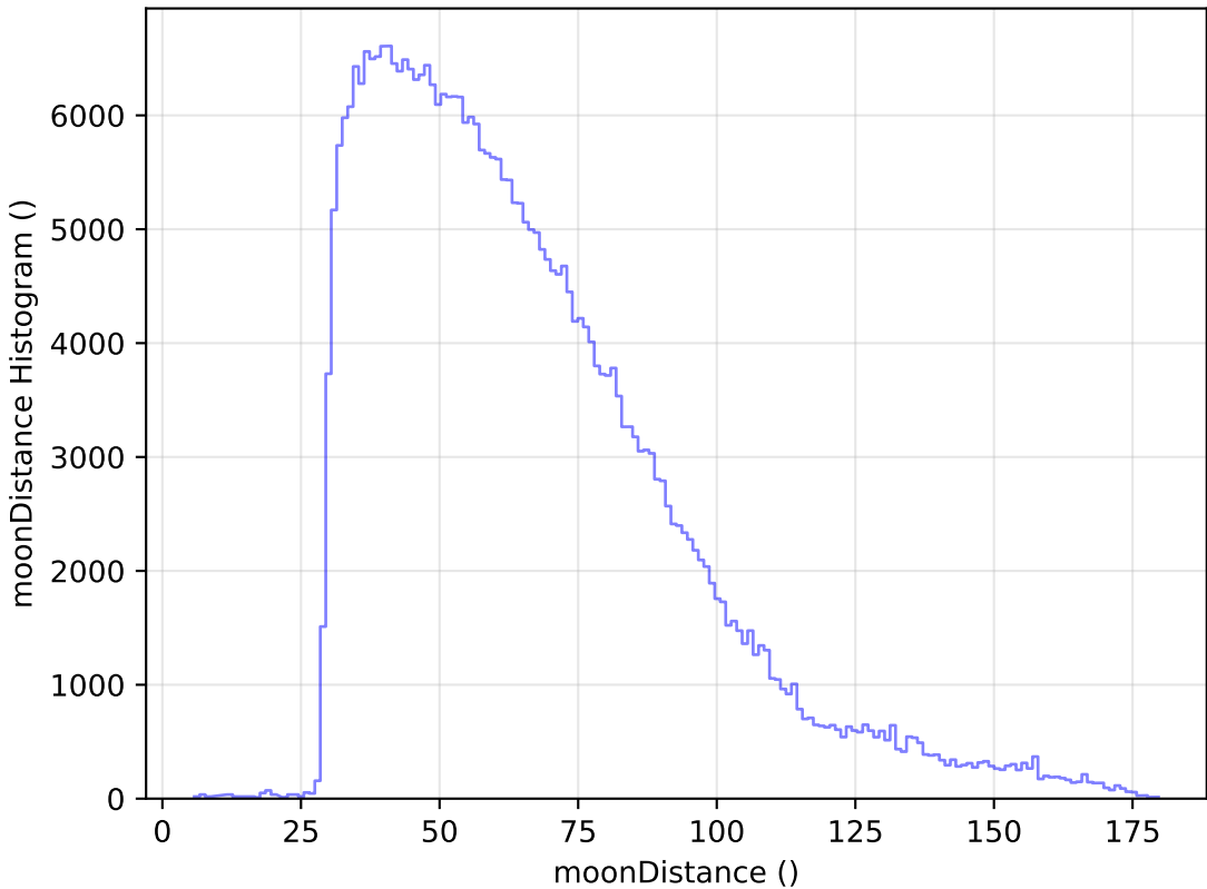
too_ignore_100_4v3.4_10yrs WFD y band: moonDistance Histogram
