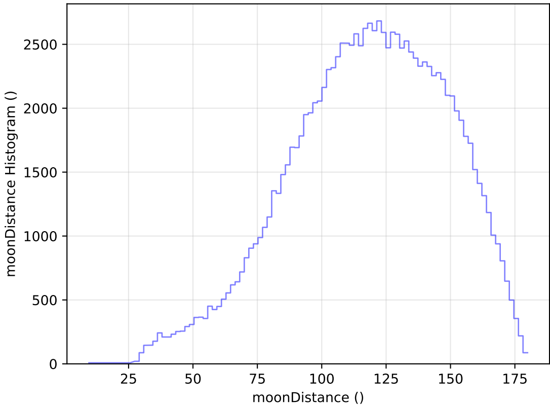
too_ignore_100_4v3.4_10yrs WFD u band: moonDistance Histogram
