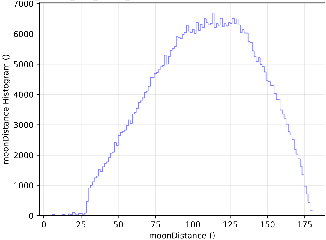
too_ignore_100_4v3.4_10yrs WFD r band: moonDistance Histogram
