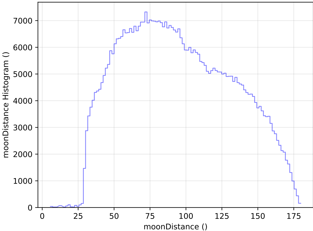
too_ignore_100_4v3.4_10yrs WFD i band: moonDistance Histogram
