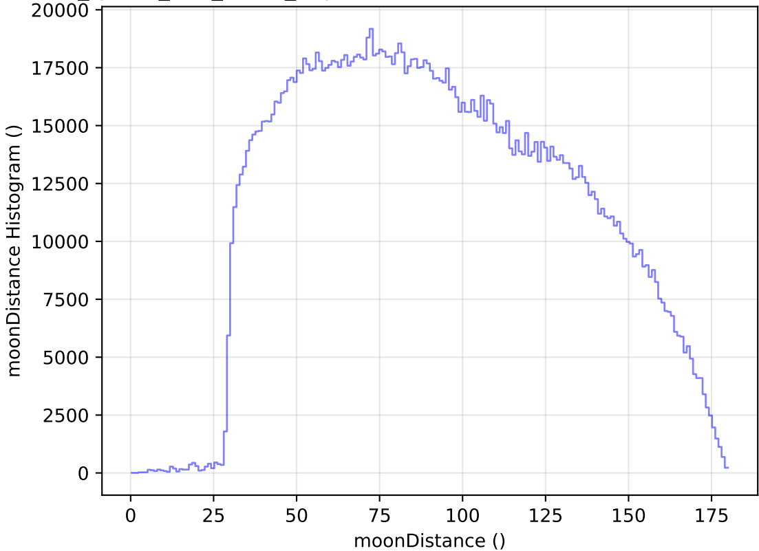
too_ignore_100_4v3.4_10yrs WFD all bands: moonDistance Histogram
