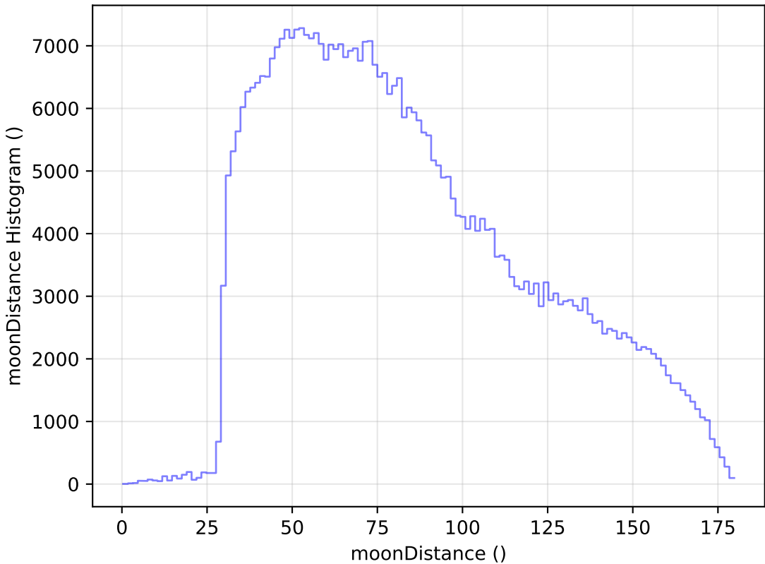
too_ignore_100_4v3.4_10yrs All sky z band: moonDistance Histogram
