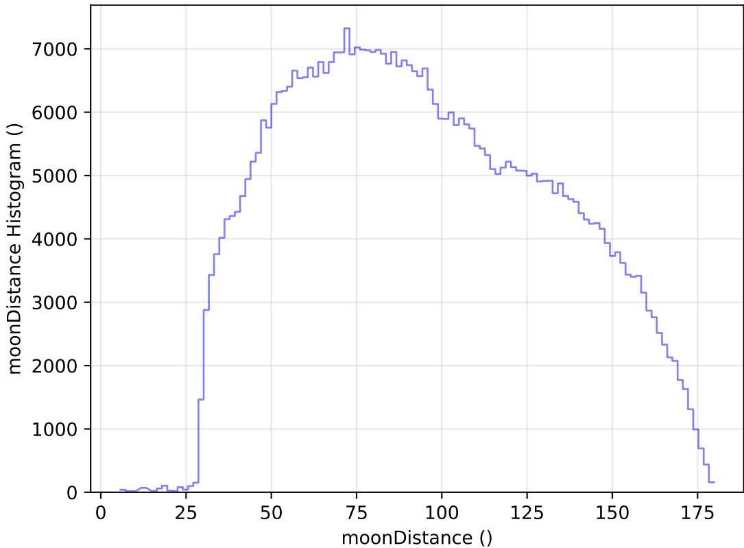
too_ignore_100_4v3.4_10yrs All sky i band: moonDistance Histogram
