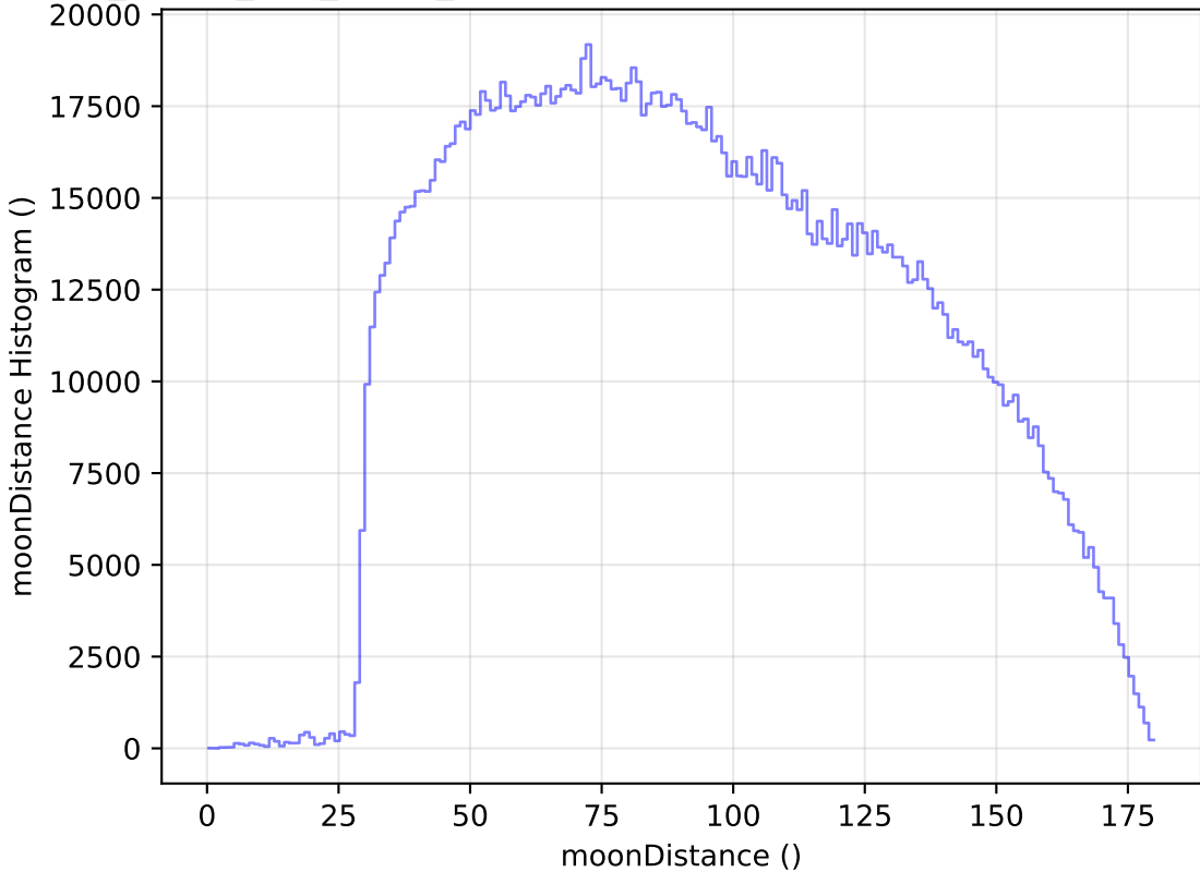
too_ignore_100_4v3.4_10yrs All sky all bands: moonDistance Histogram
