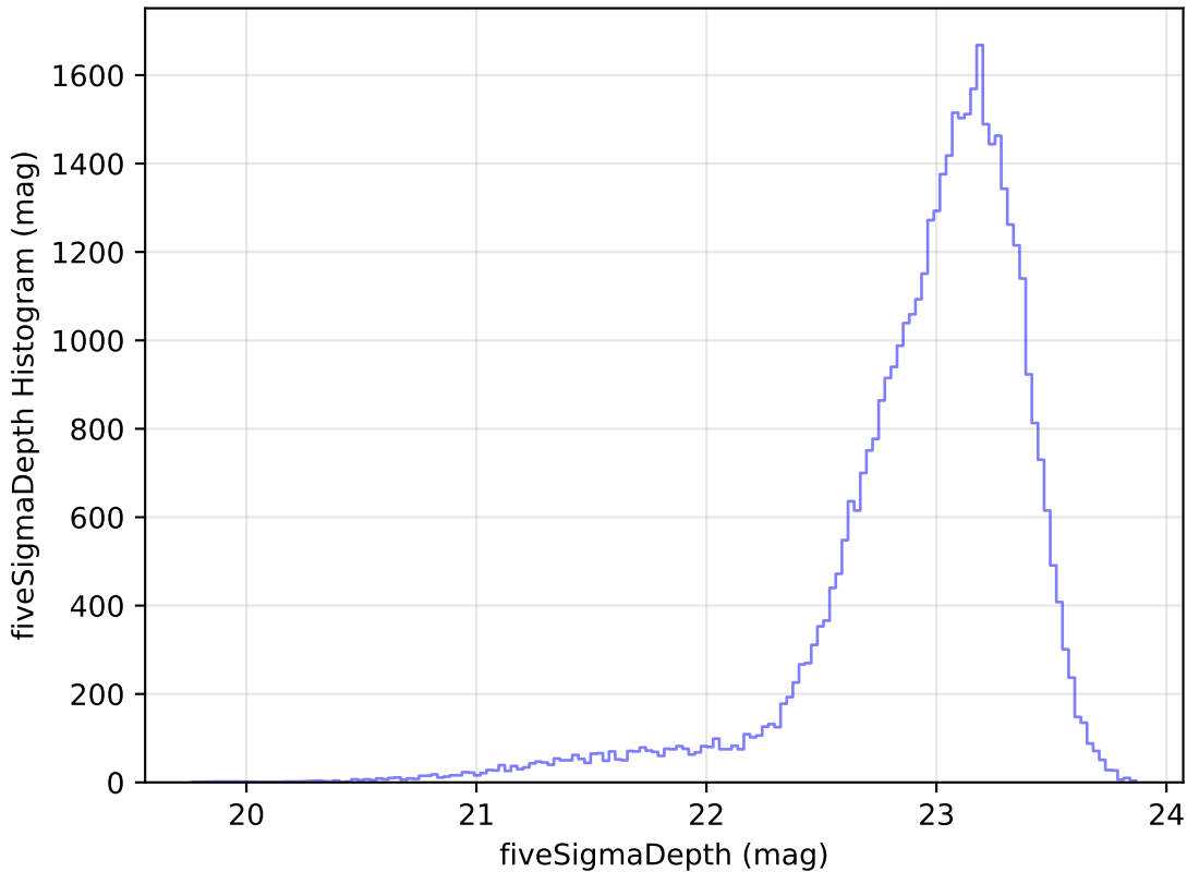
too_ignore_100_4v3.4_10yrs Yr 1 z band: fiveSigmaDepth Histogram
