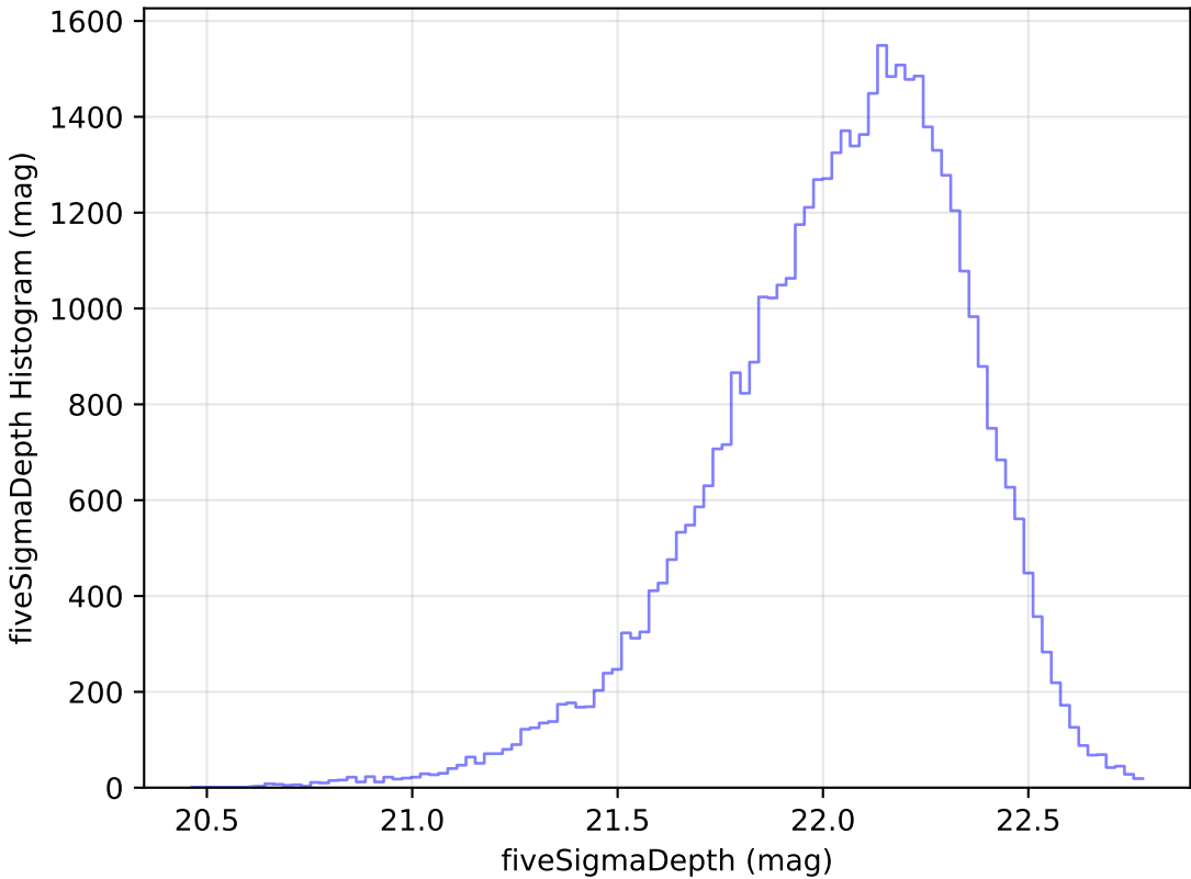
too_ignore_100_4v3.4_10yrs Yr 1 y band: fiveSigmaDepth Histogram
