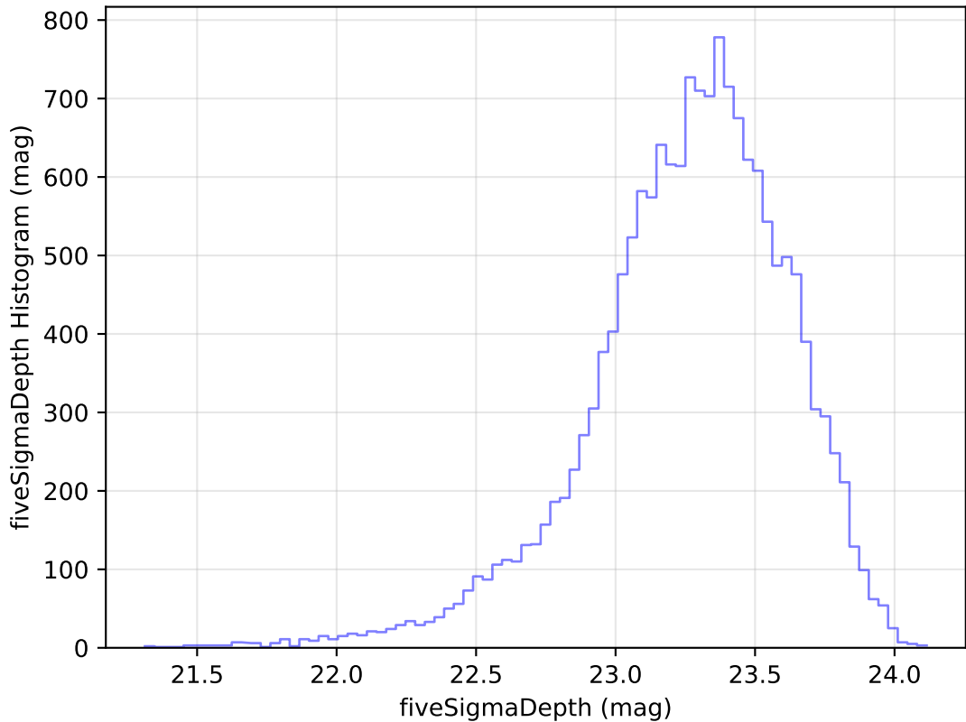
too_ignore_100_4v3.4_10yrs Yr 1 u band: fiveSigmaDepth Histogram
