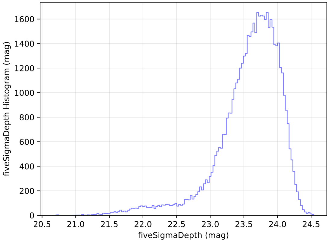
too_ignore_100_4v3.4_10yrs Yr 1 i band: fiveSigmaDepth Histogram
