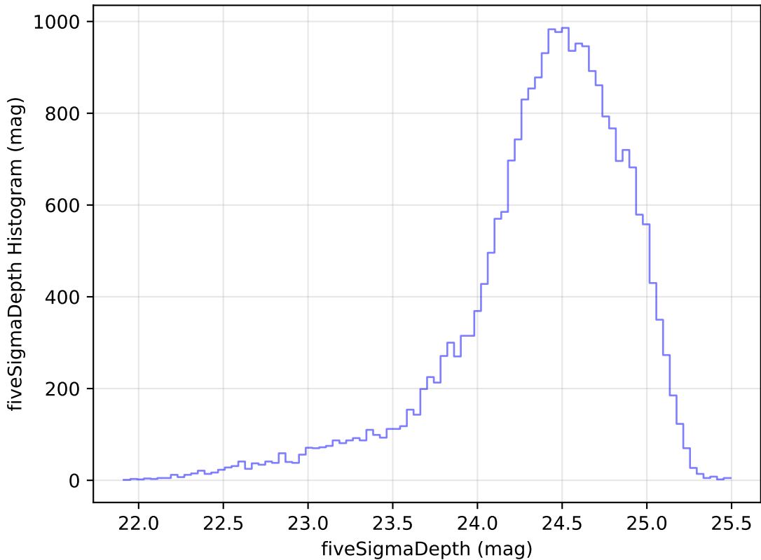
too_ignore_100_4v3.4_10yrs Yr 1 g band: fiveSigmaDepth Histogram
