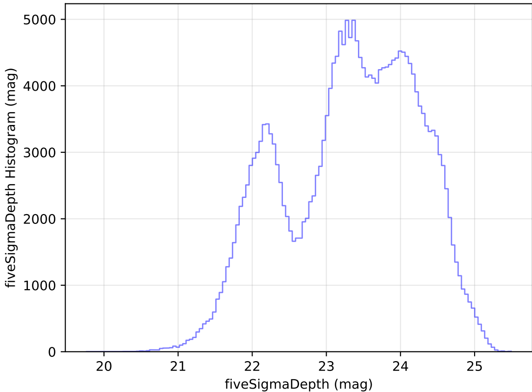
too_ignore_100_4v3.4_10yrs Yr 1 all bands: fiveSigmaDepth Histogram
