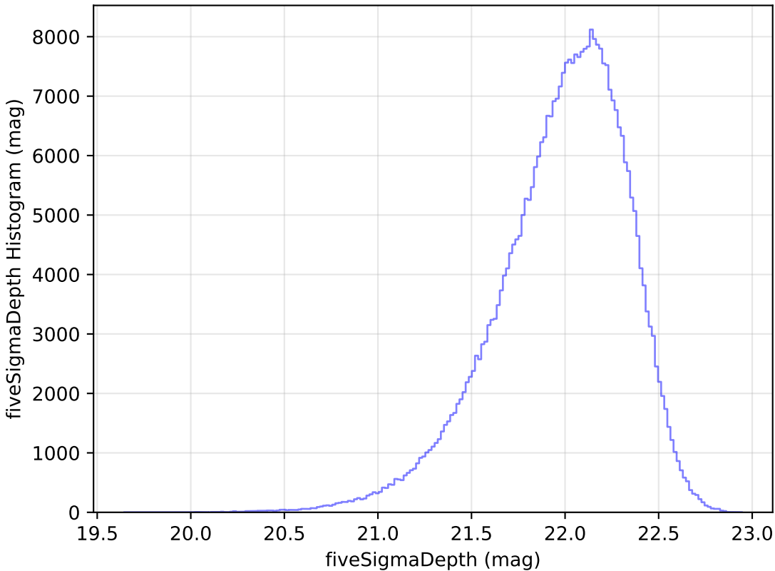
too_ignore_100_4v3.4_10yrs WFD y band: fiveSigmaDepth Histogram
